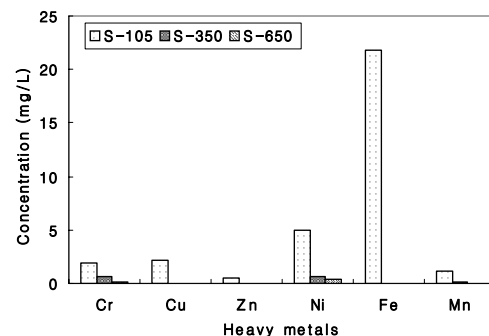
Fig. 2. Heavy metal leaching concentration by KLT method.
