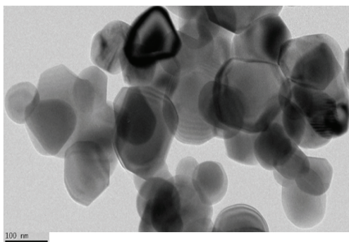
Fig. 4. SEM micrograph of \text{TiO}_2/\text{MMA} core-shell polymer(EU-S133D 0.5g).
