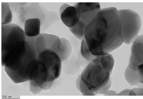
Fig. 5. SEM micrograph of \text{TiO}_2/\text{MMA} core-shell polymer(EU-S133D 4.0g).
