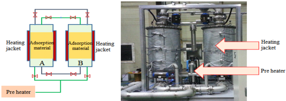
Fig. 4. Schematic diagram of VOCs concentrator.
