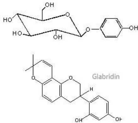
Fig. 1. Structures of Arbutin and Glabridin
