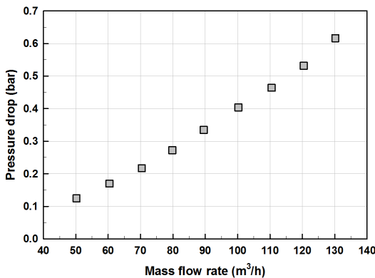
Fig. 9. Pressure drop of water side.
