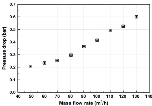
Fig. 11. Pressure drop of oil side.
