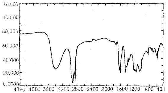
Fig. 1. IR Spectrum of the mixture
