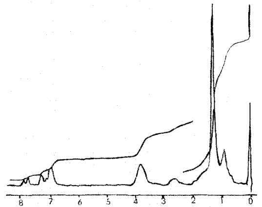
Fig. 3. Proton NMR Spectrum of the mixture in \text{CCl}_4
